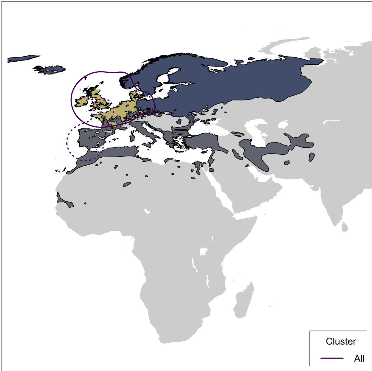
Figure 10110-1. Map showing 95% kernel contours of of first-level clusters identified by the migratory connectivity analysis, if any, or 95% kernel contours of all encounters, in case of no clustering structure. Solid lines indicate the clusters in the breeding range, dotted lines those in the non-breeding range. Different contour colours correspond to different clusters, as reported in legend. The species distribution range is also shown (breeding range: blue; non-breeding range: dark grey; resident range: beige; from BirdLife International, 2019).
