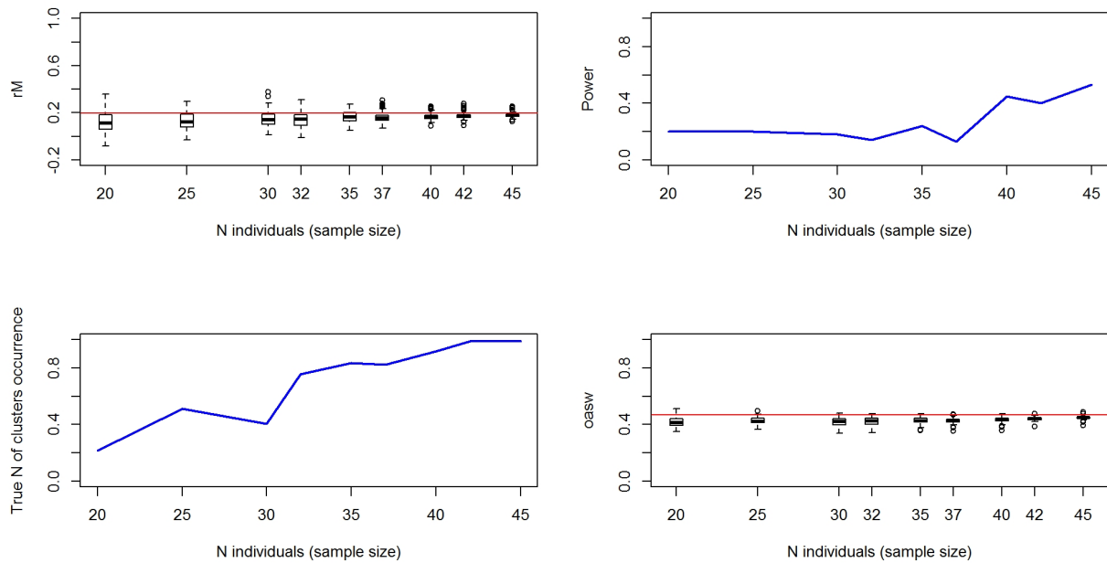
Figure 09760-3. Top left: simulated distribution (boxplots) and observed value (red line) of connectivity. Top right: Simulated power of the analysis. Bottom left: Proportion of times the analysis provides the
