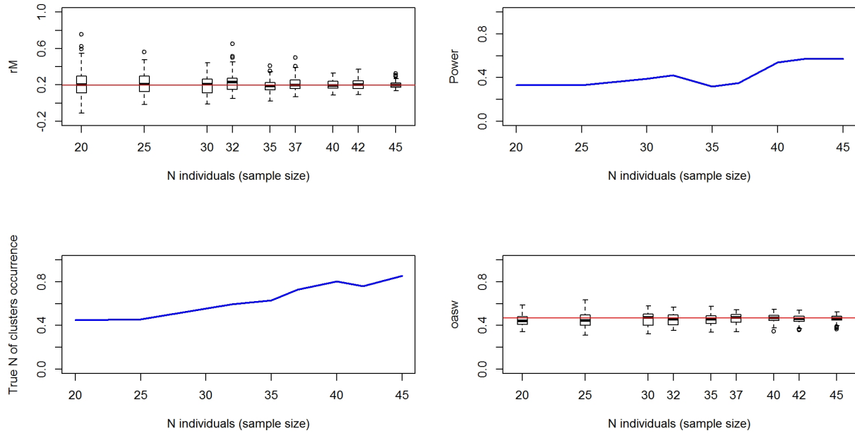
Figure 09760-2. Top left: simulated distribution (boxplots) and observed value (red line) of connectivity. Top right: Simulated power of the analysis (i.e. proportion of times the analyses on the subset of individuals was significant). Bottom left: Proportion of times the analysis provides the observed best number of cluster. Bottom right: simulated distribution (boxplots) and observed value (red line) of clustering intensity.
