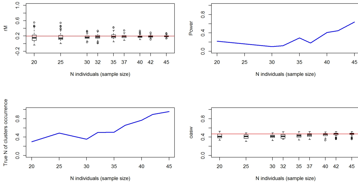
Figure 09760-4. Top left: simulated distribution (boxplots) and observed value (red line) of connectivity. Top right: Simulated power of the analysis. Bottom left: Proportion of times the analysis provides the observed best number of cluster. Bottom right: simulated distribution (boxplots) and observed value (red line) of clustering intensity.
