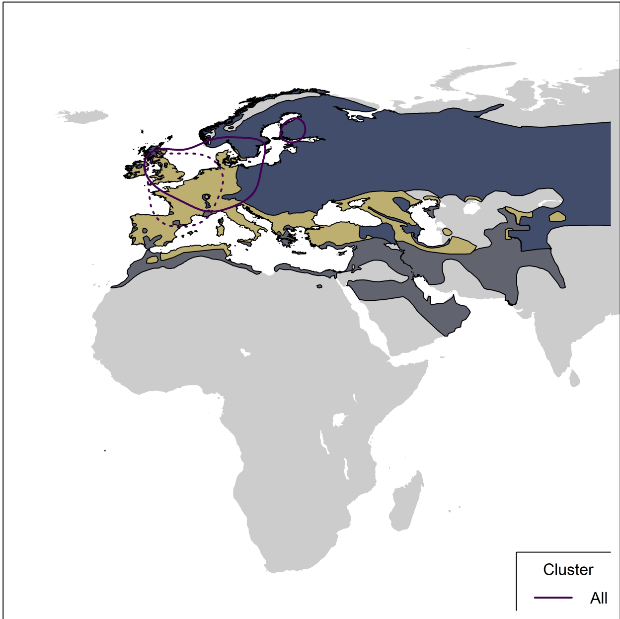
Figure 09760-1. Map showing 95% kernel contours of of first-level clusters identified by the migratory connectivity analysis, if any, or 95% kernel contours of all encounters, in case of no clustering structure. Solid lines indicate the clusters in the breeding range, dotted lines those in the non-breeding range. Different contour colours correspond to different clusters, as reported in legend. The species distribution range is also shown (breeding range: blue; non-breeding range: dark grey; resident range: beige; from BirdLife International, 2019).
