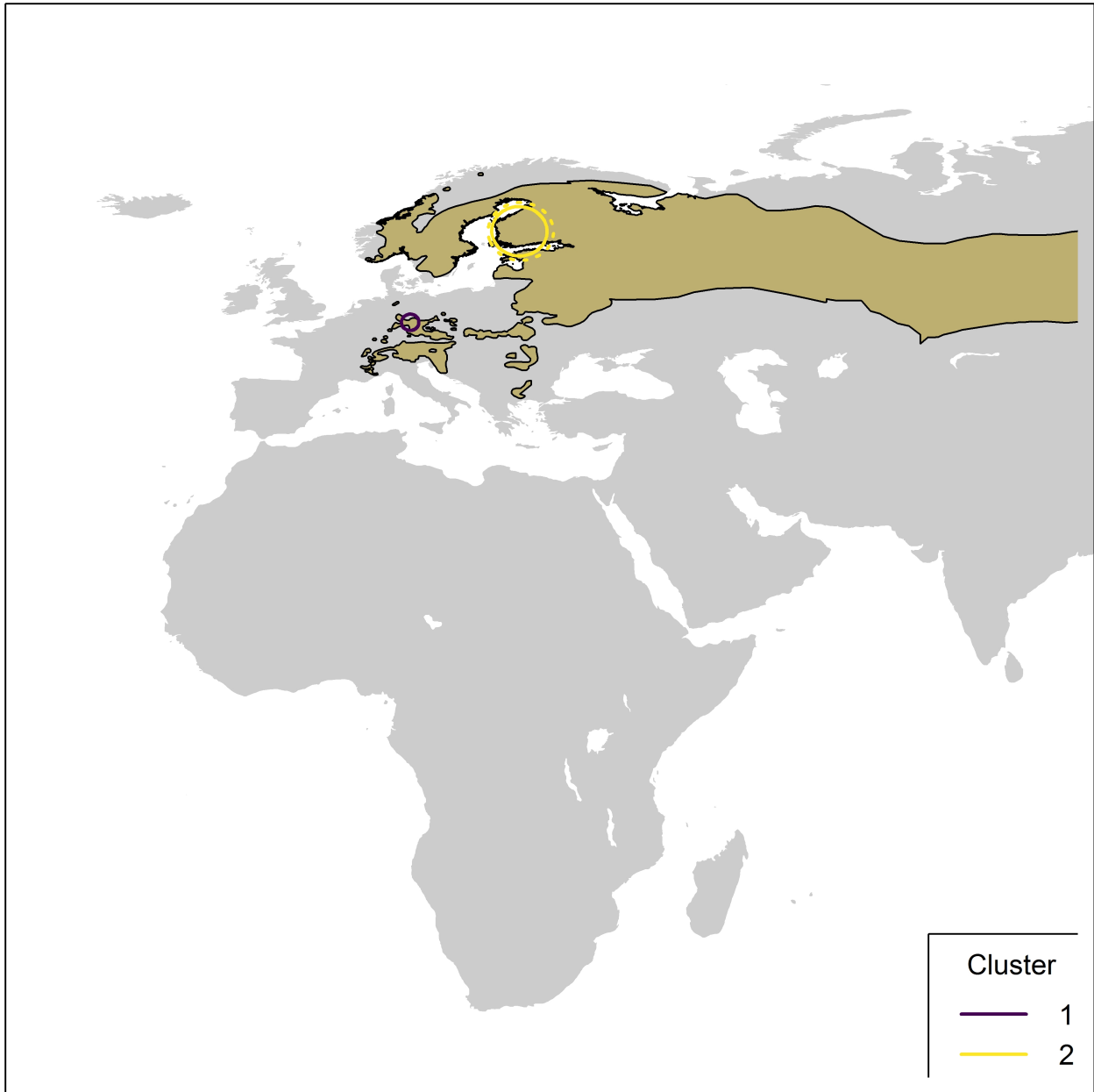
Figure 07510-1. Map showing 95% kernel contours of of first-level clusters identified by the migratory connectivity analysis, if any, or 95% kernel contours of all encounters, in case of no clustering structure. Solid lines indicate the clusters in the breeding range, dotted lines those in the non-breeding range. Different contour colours correspond to different clusters, as reported in legend. The species distribution range is also shown (breeding range: blue; non-breeding range: dark grey; resident range: beige; from BirdLife International, 2019).
