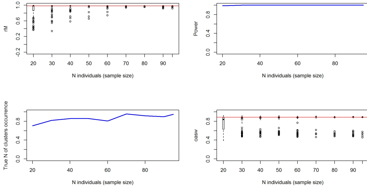
Figure 07510-2. Top left: simulated distribution (boxplots) and observed value (red line) of connectivity. Top right: Simulated power of the analysis (i.e. proportion of times the analyses on the subset of individuals was significant). Bottom left: Proportion of times the analysis provides the observed best number of cluster. Bottom right: simulated distribution (boxplots) and observed value (red line) of clustering intensity.
