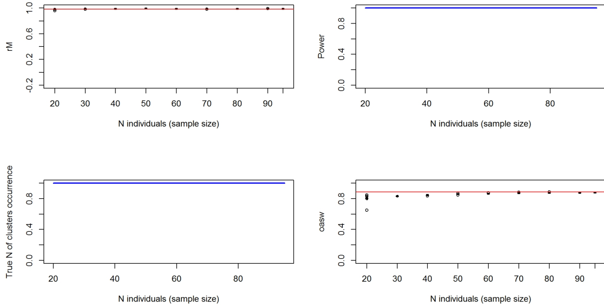
Figure 07510-4. Top left: simulated distribution (boxplots) and observed value (red line) of connectivity. Top right: Simulated power of the analysis. Bottom left: Proportion of times the analysis provides the observed best number of cluster. Bottom right: simulated distribution (boxplots) and observed value (red line) of clustering intensity.
