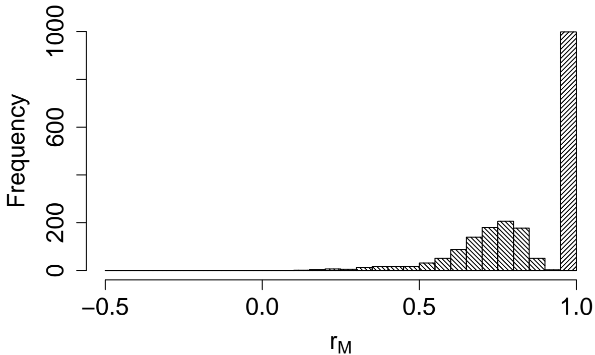
Figure 07510-5. Comparison between the bootstrapped distributions of connectivity value for alive recaptures (filling lines with angle=45°) and dead recoveries (filling lines with angle=375°).
