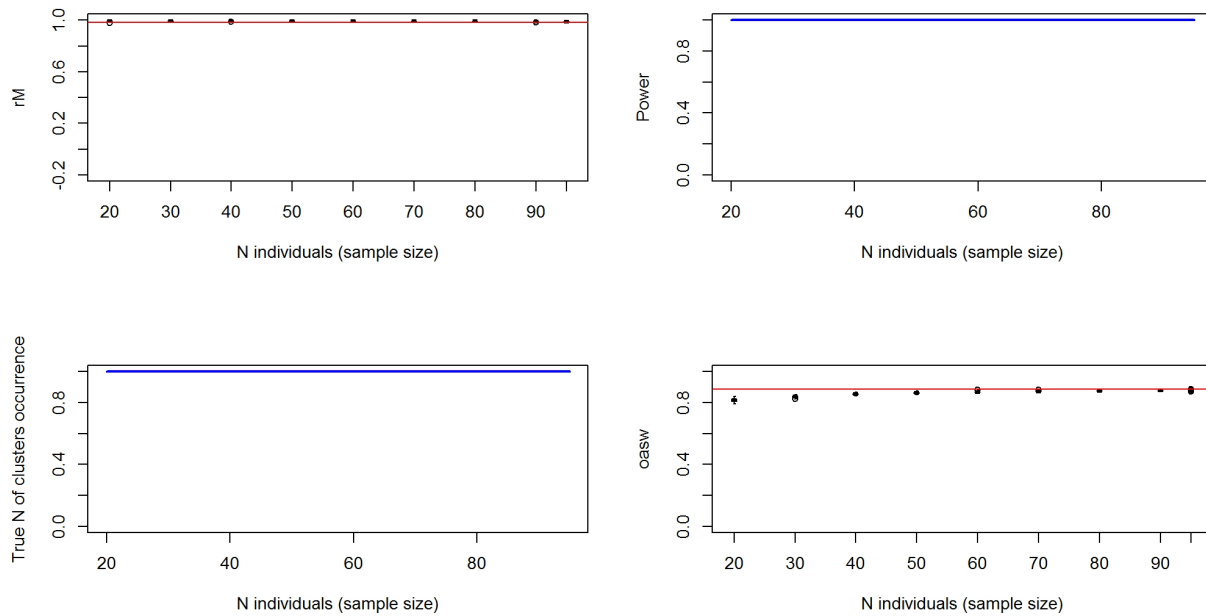
Figure 07510-3. Top left: simulated distribution (boxplots) and observed value (red line) of connectivity. Top right: Simulated power of the analysis. Bottom left: Proportion of times the analysis provides the
