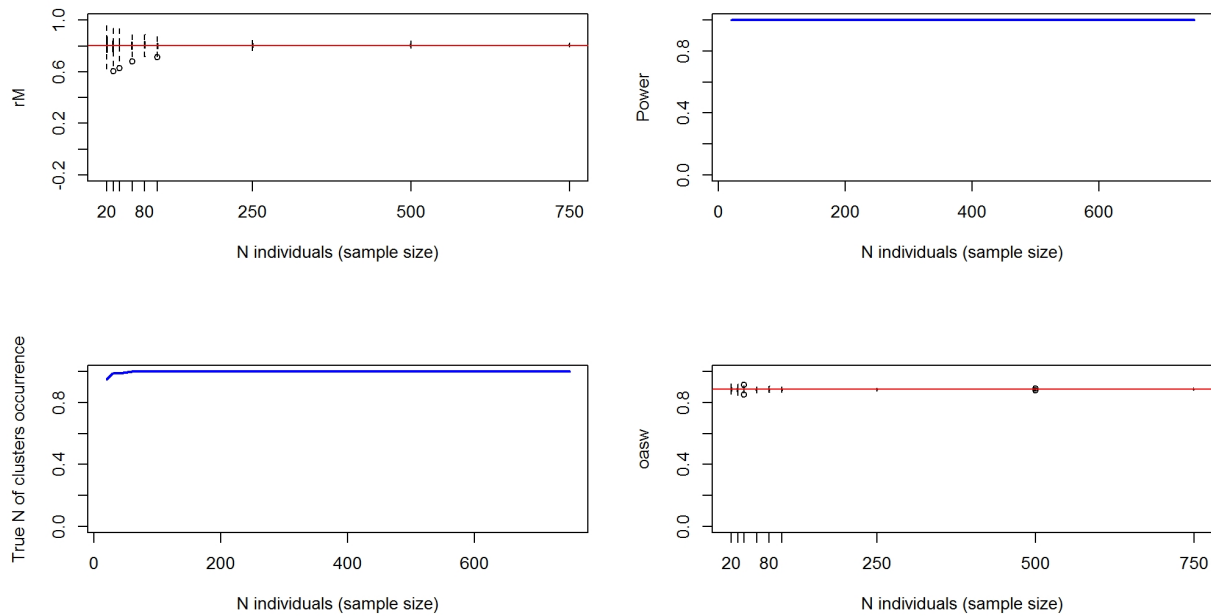
Figure 01580-3. Top left: simulated distribution (boxplots) and observed value (red line) of connectivity. Top right: Simulated power of the analysis. Bottom left: Proportion of times the analysis provides the
