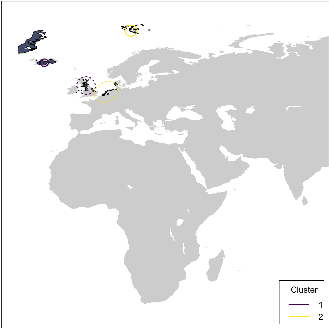
Figure 01580-1. Map showing 95% kernel contours of of first-level clusters identified by the migratory connectivity analysis, if any, or 95% kernel contours of all encounters, in case of no clustering structure. Solid lines indicate the clusters in the breeding range, dotted lines those in the non-breeding range. Different contour colours correspond to different clusters, as reported in legend. The species distribution range is also shown (breeding range: blue; non-breeding range: dark grey; resident range: beige; from BirdLife International, 2019).
