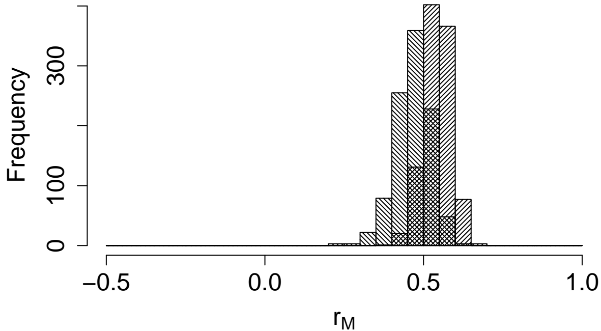
Figure 01580-5. Comparison between the bootstrapped distributions of connectivity value for alive recaptures (filling lines with angle=45°) and dead recoveries (filling lines with angle=375°).
