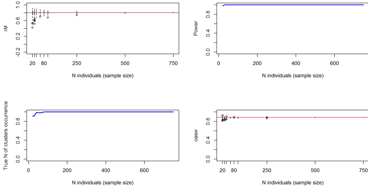
Figure 01580-4. Top left: simulated distribution (boxplots) and observed value (red line) of connectivity. Top right: Simulated power of the analysis. Bottom left: Proportion of times the analysis provides the observed best number of cluster. Bottom right: simulated distribution (boxplots) and observed value (red line) of clustering intensity.
