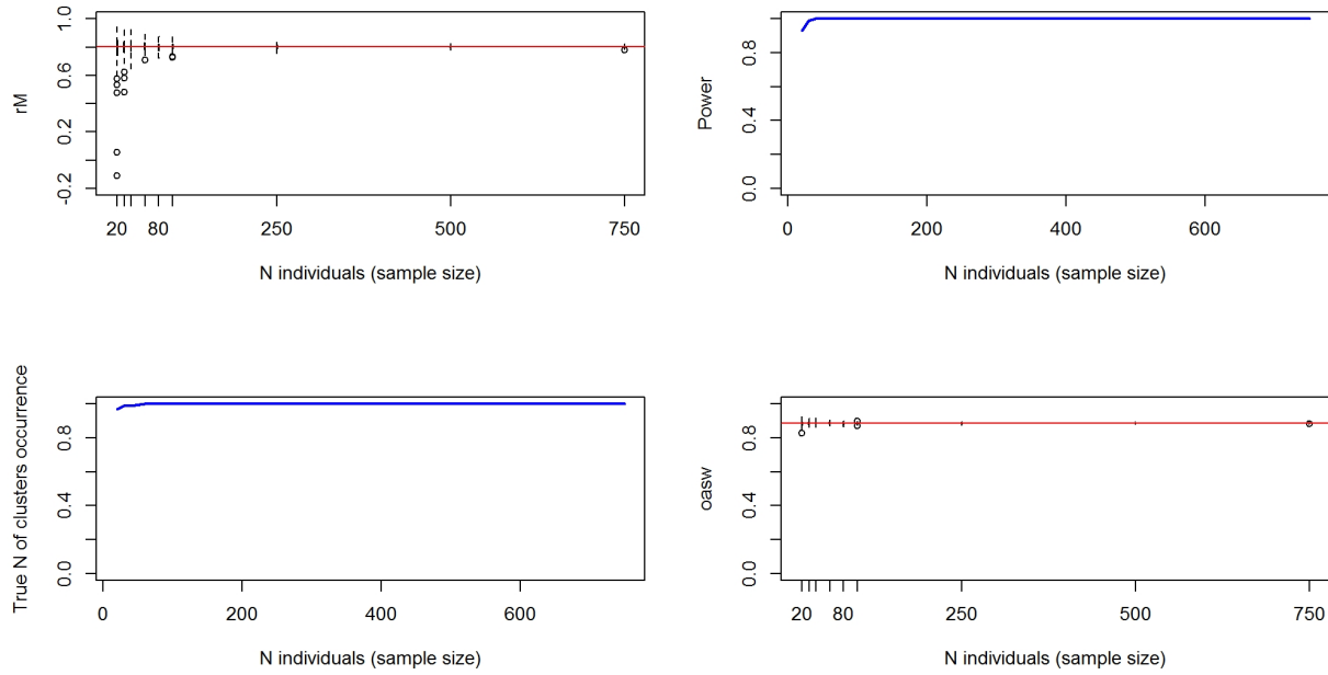
Figure 01580-2. Top left: simulated distribution (boxplots) and observed value (red line) of connectivity. Top right: Simulated power of the analysis (i.e. proportion of times the analyses on the subset of individuals was significant). Bottom left: Proportion of times the analysis provides the observed best number of cluster. Bottom right: simulated distribution (boxplots) and observed value (red line) of clustering intensity.
